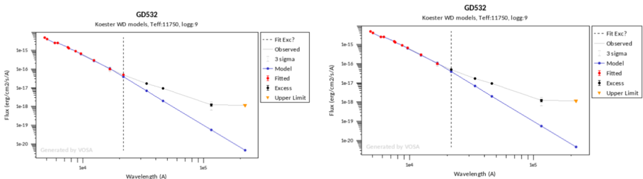
Figure 8. Plot of the SED fitting before and after refining the infrared excess ( Step 8 ).
